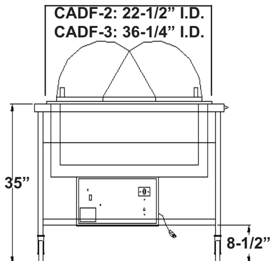
REAR ELEVATION
